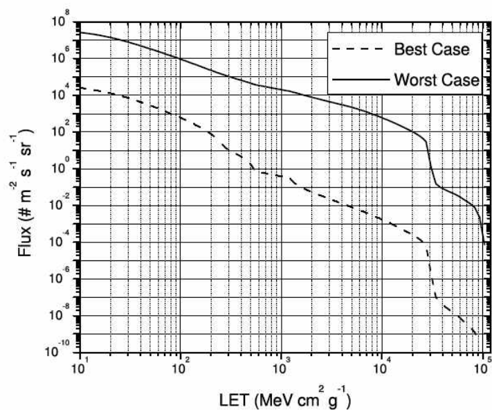
Figure 3-6 Charged particle flux under 2 mm aluminum shielding
